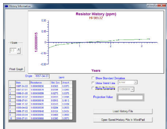
Resistor History
