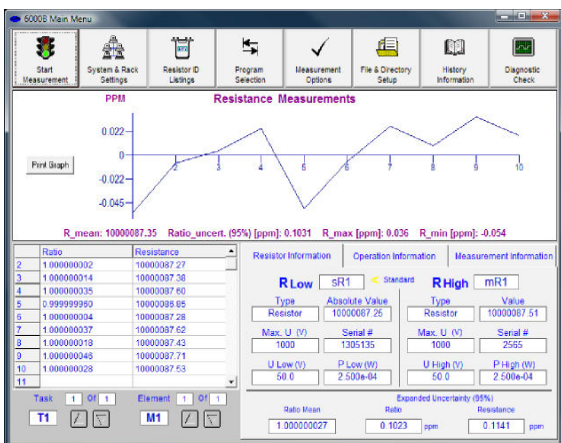
Main Menu
