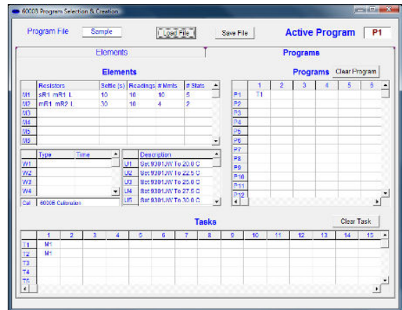
Program Selection
