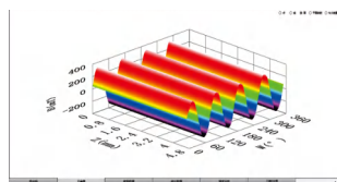
3D Distribution Map of Surface Magnetism
